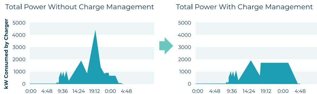
Figure 10: Managed Charging Can Decrease Peak Power Demand
